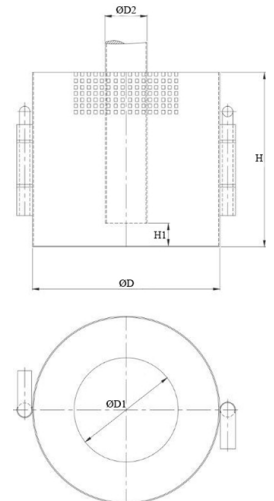
482670 Suction strainer
