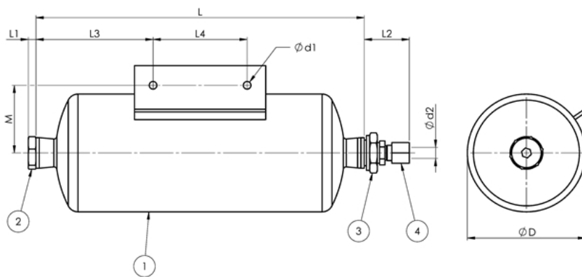
Header tank
