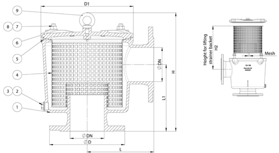
482751 Mudbox Measurement drawing
