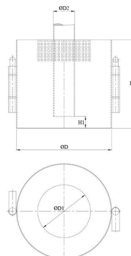
482670 Suction strainer
